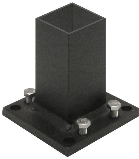
STANDARD 2" POST .090 Wall \frac{3}{8}" \text{ h } \times 3\frac{7}{8}" \text{ sq. plate }
